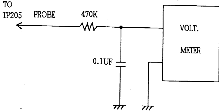
FIGURE 4 CONNECTION DIAGRAM
