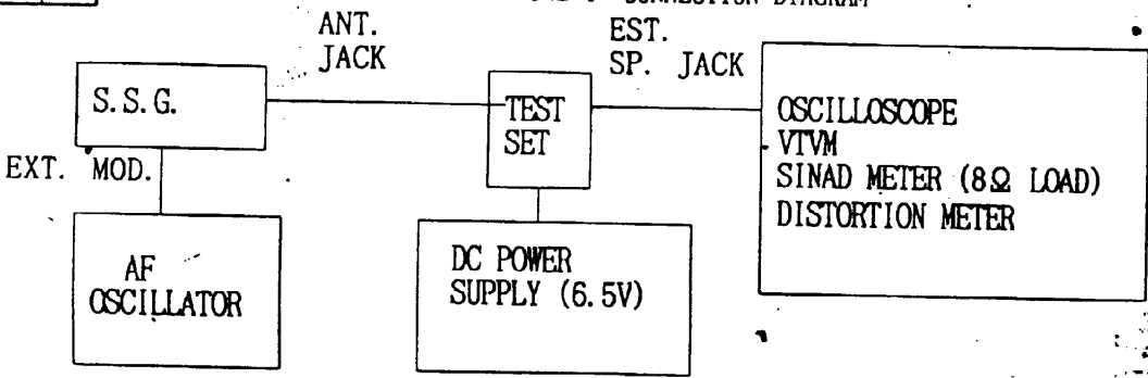
FIGURE 4 CONNECTION DIAGRAM
